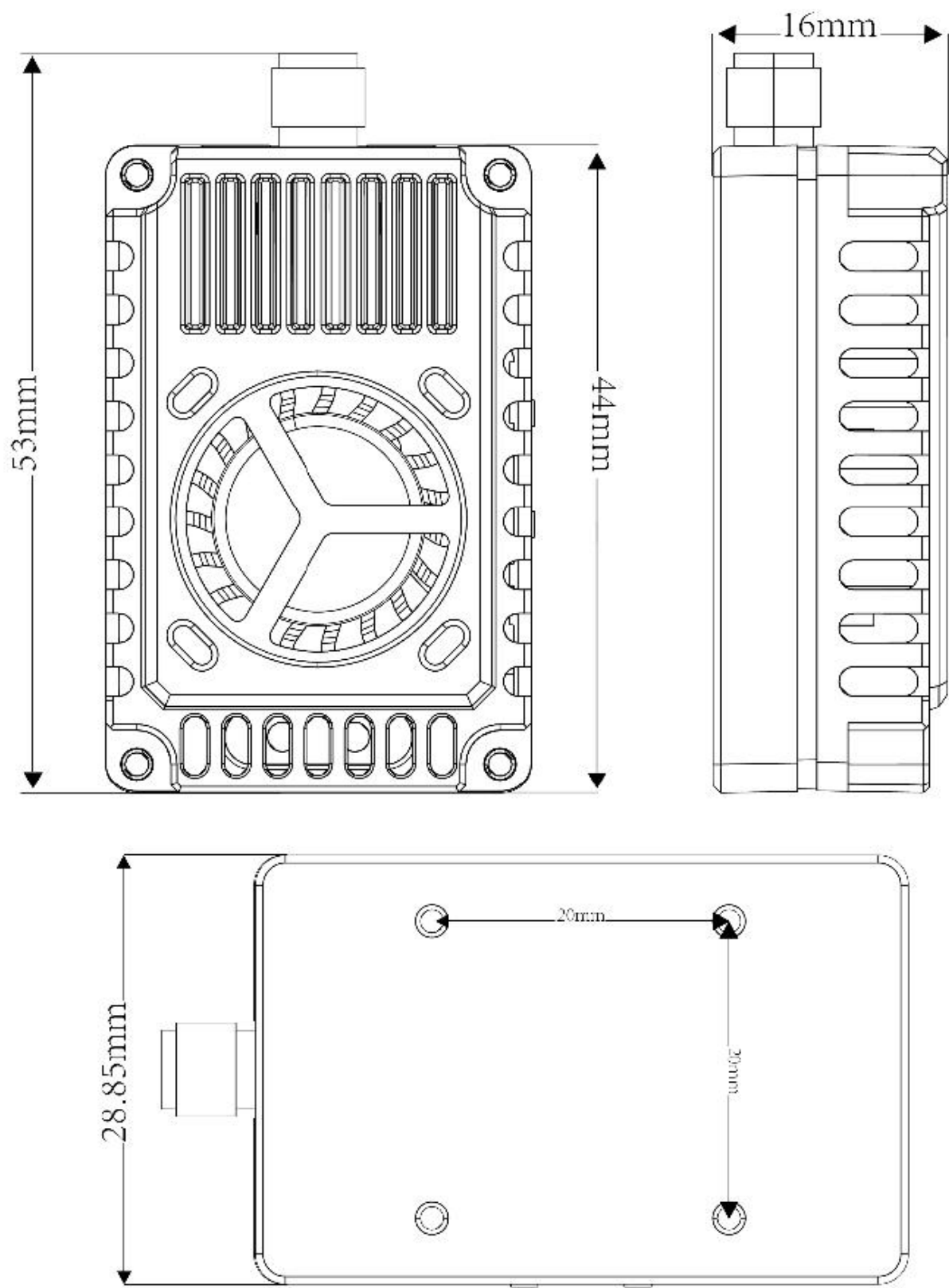
Dimensions and mounting-hole layout. Unit: mm.
